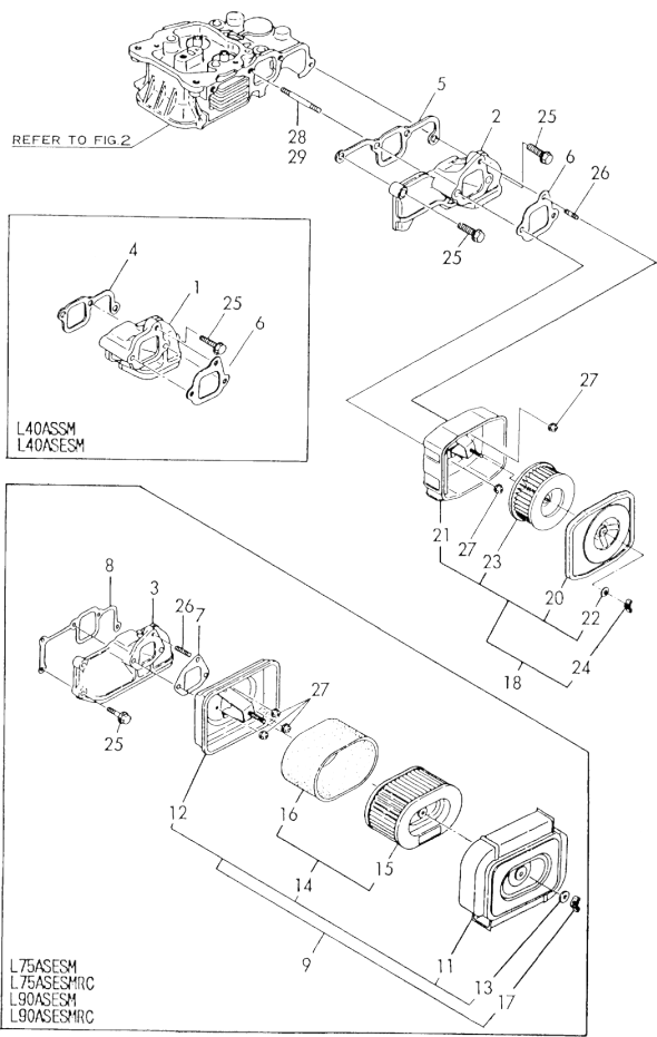
Fig.3. AIR CLEANER
