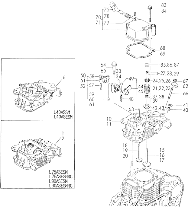
Fig.2. CYLINDER HEAD & BONNET
