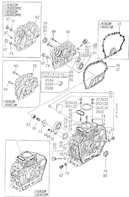
Fig.1. CYLINDER BLOCK
