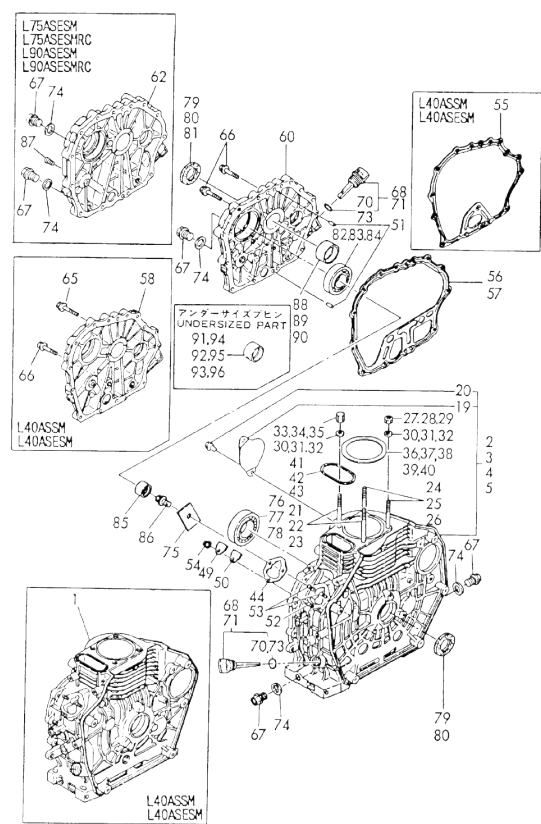
Fig.1. CYLINDER BLOCK
